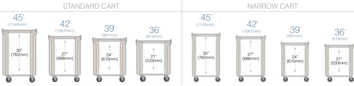
Nominal dimensions shown above
